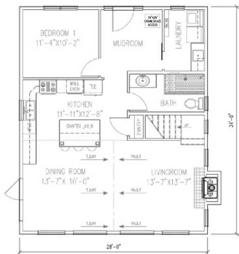
MAIN FLOOR PLAN SCALE: \frac{1}{8} "=1'-0"
